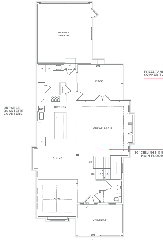
MAIN FLOOR 1327 SQFT
