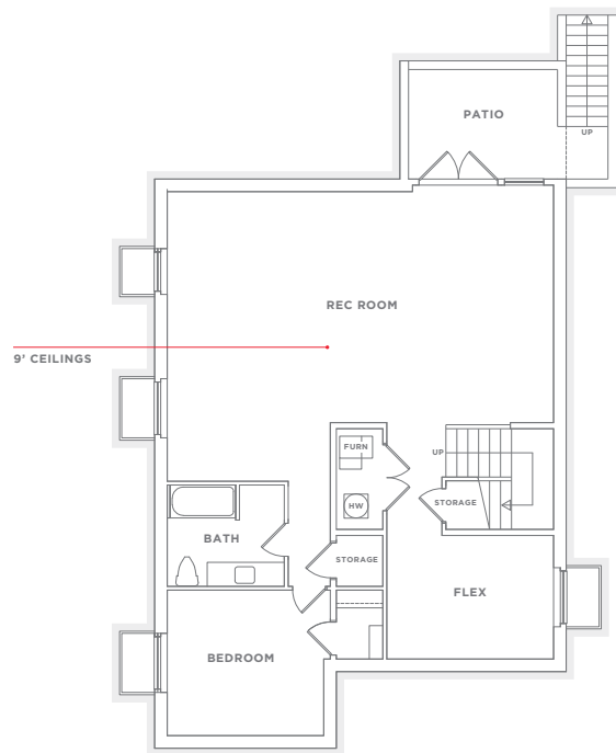
LOWER FLOOR 1,256 SQFT APPROX.
